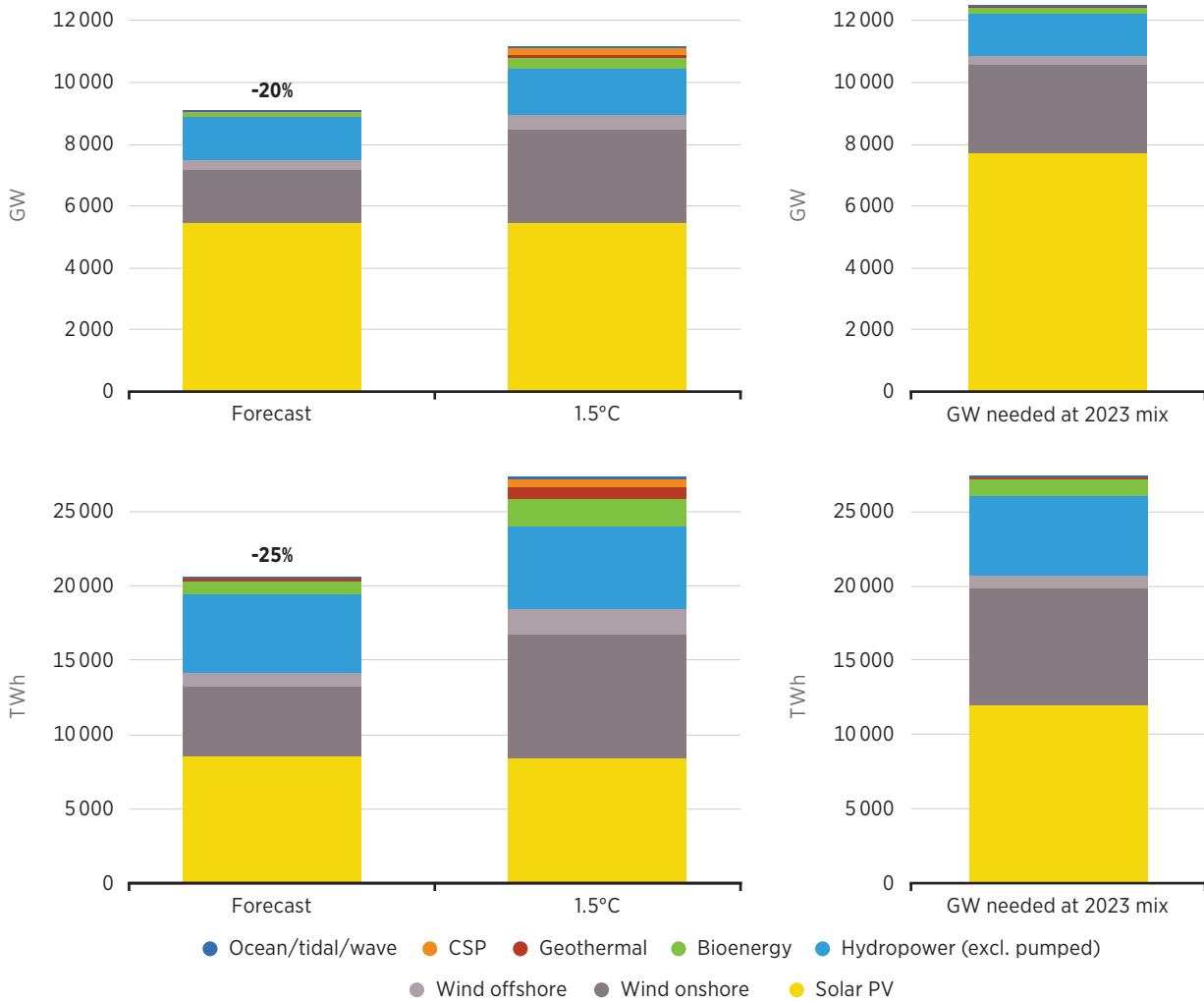
Figure 11 Global electricity generation under the tripling goal compared to current expectations, 2030
