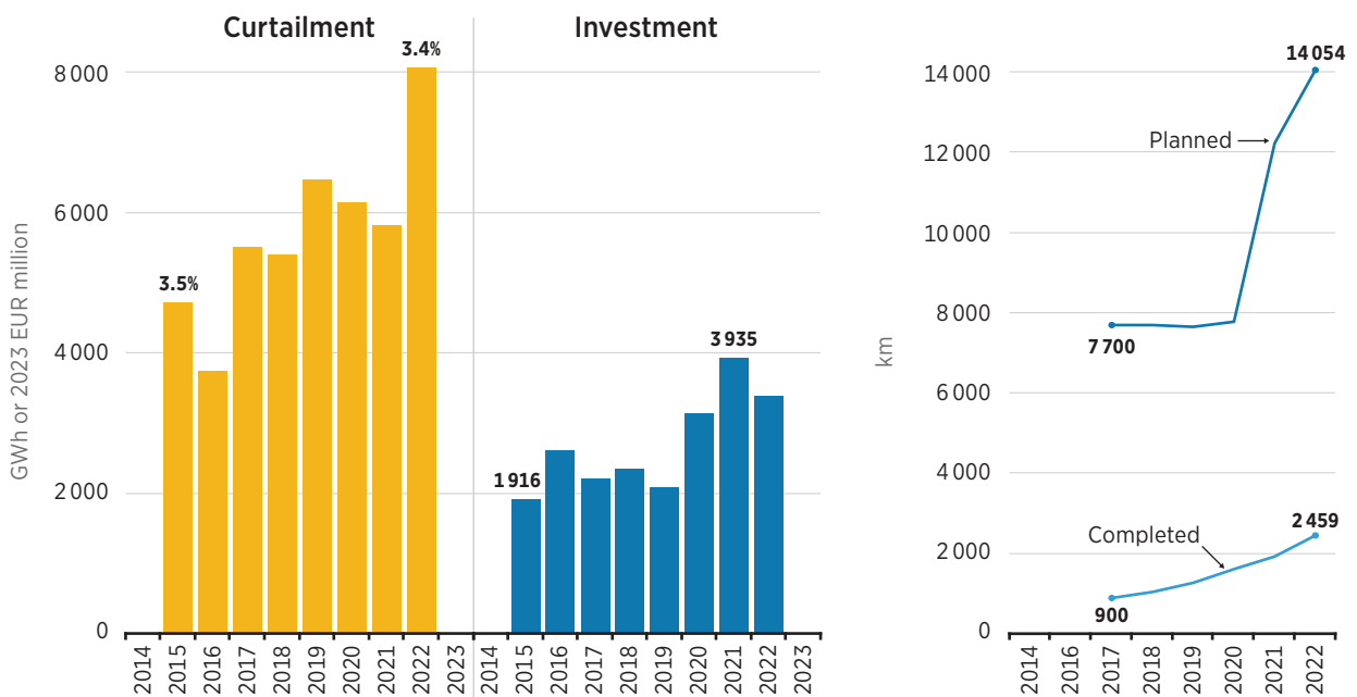
Figure 14 Grid curtailment of solar and wind, transmission network investment and planned and completed line length for Germany, 2015-2022
