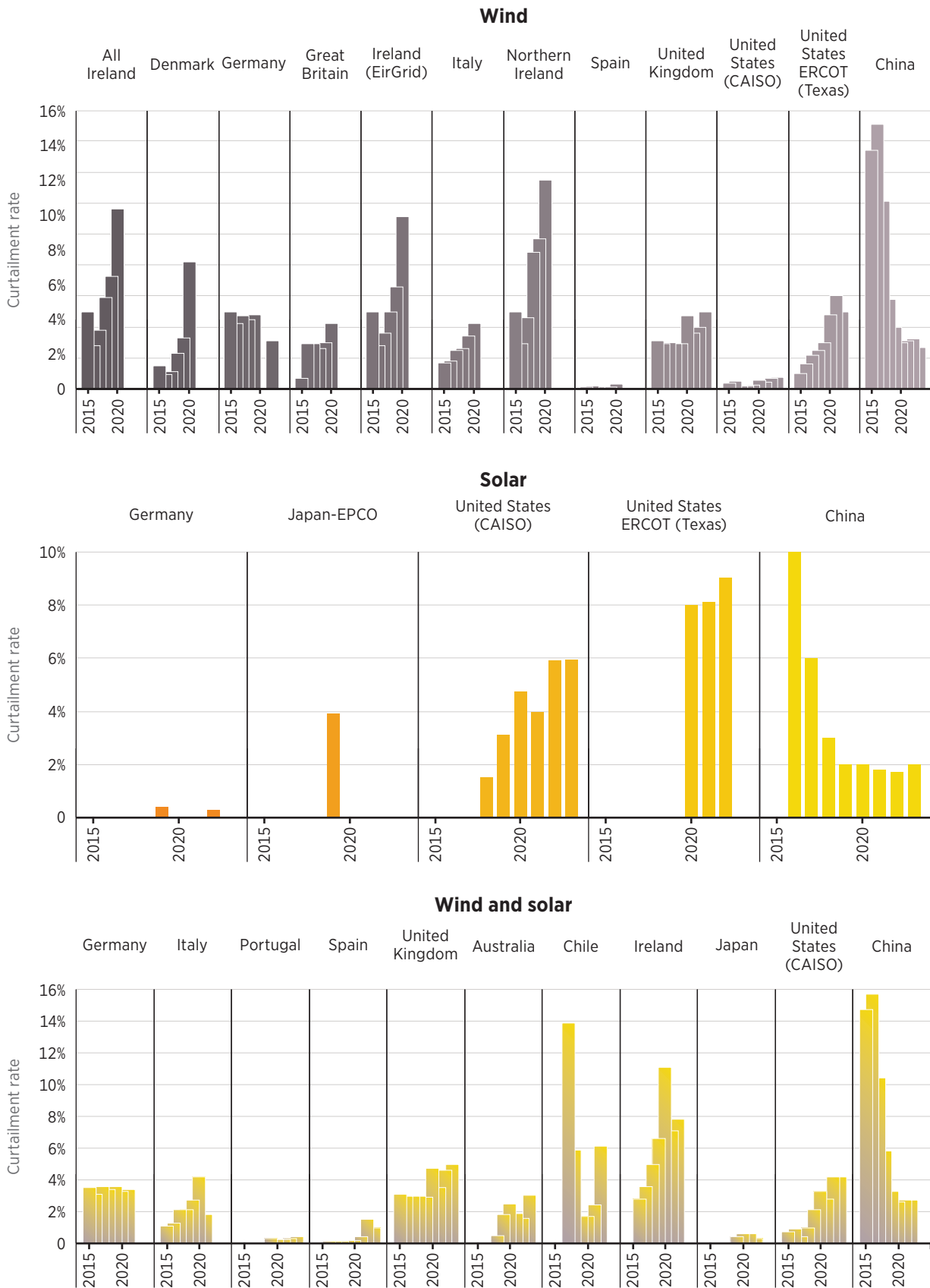
Figure 13 Curtailment rates for solar, wind and variable renewable electricity by country, 2015-2023
