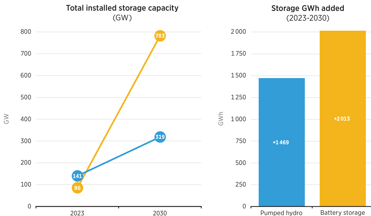
Figure 19 Projected battery storage growth and required pumped hydropower capacity growth to 2030
