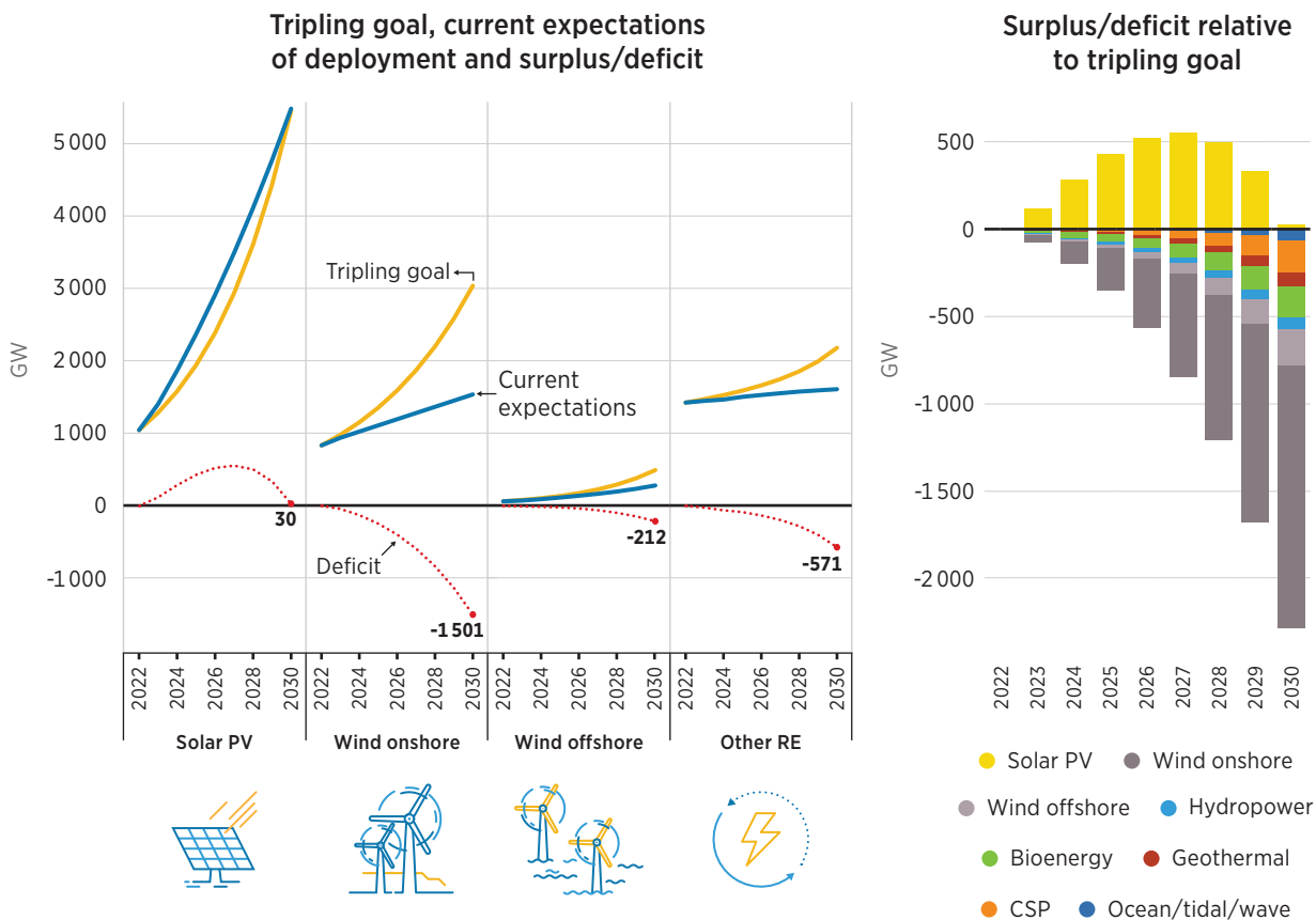
Figure 9 Current expectations of global cumulative renewable power capacity to 2030 compared to the tripling goal by technology, 2022-2030
