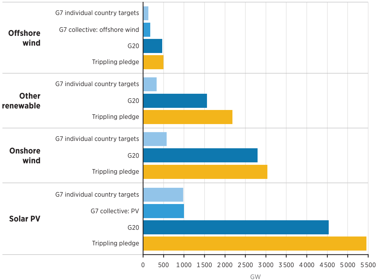
Figure 4 Individual country, regional and global renewable power targets by technology, 2030
