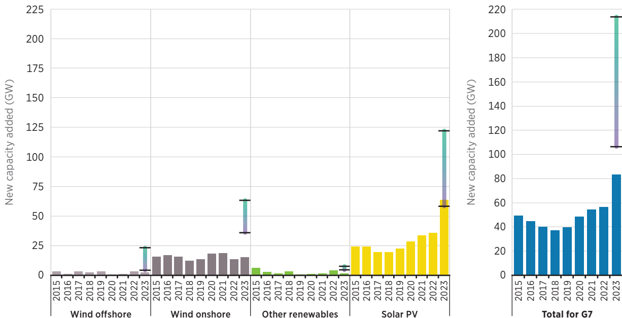
Figure 5 New capacity additions of renewable power in the G7 compared to what is required for the tripling goal in 2023, 2015 -2023
