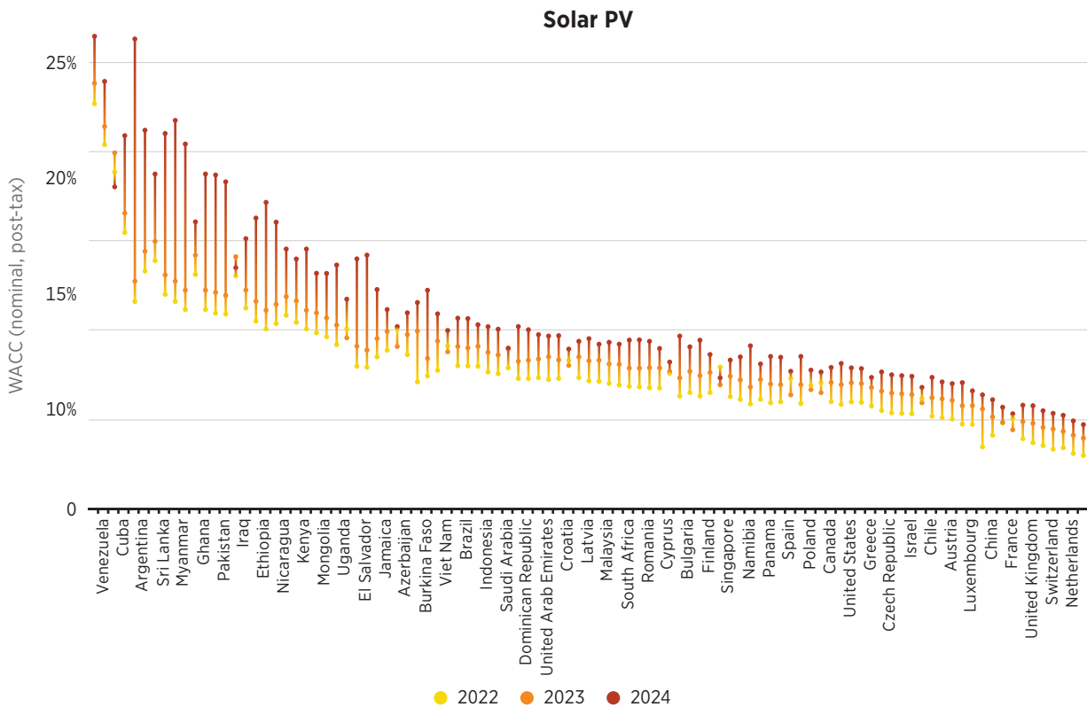
Figure 17 Nominal, post-tax weighted-average cost of capital for utility-scale solar PV projects by country, 2022-2024
