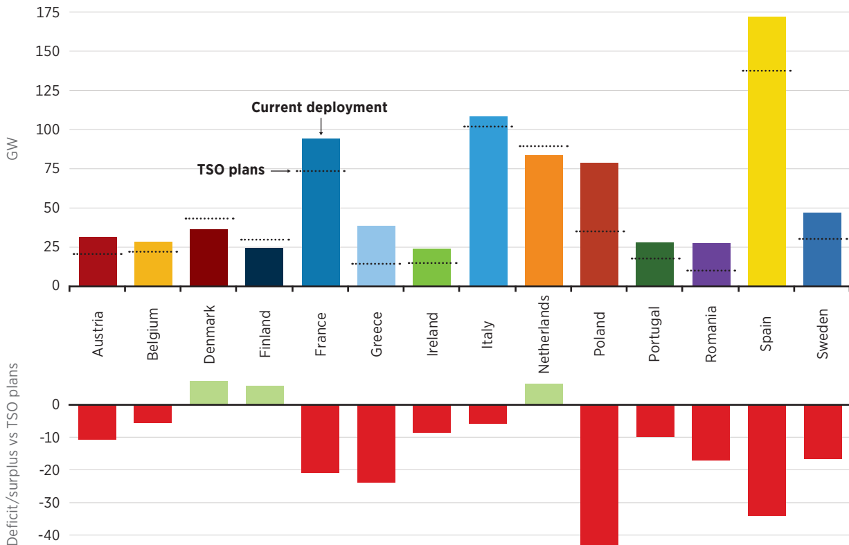
Figure 16 Anticipated solar and wind capacity in transmission system operators’ expansion plans compared to current expectations of actual deployment in 2030
